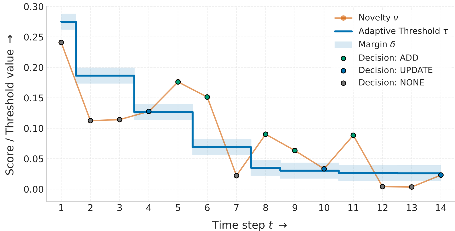
Scores and adaptive threshold over time for SAGE
