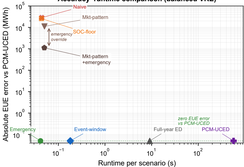
Accuracy–runtime comparison (balanced VRE)
