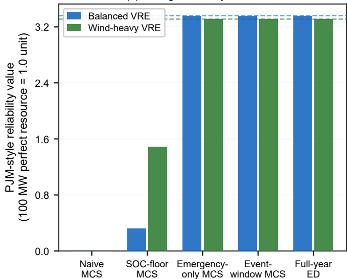
(a) Storage reliability value ratio
