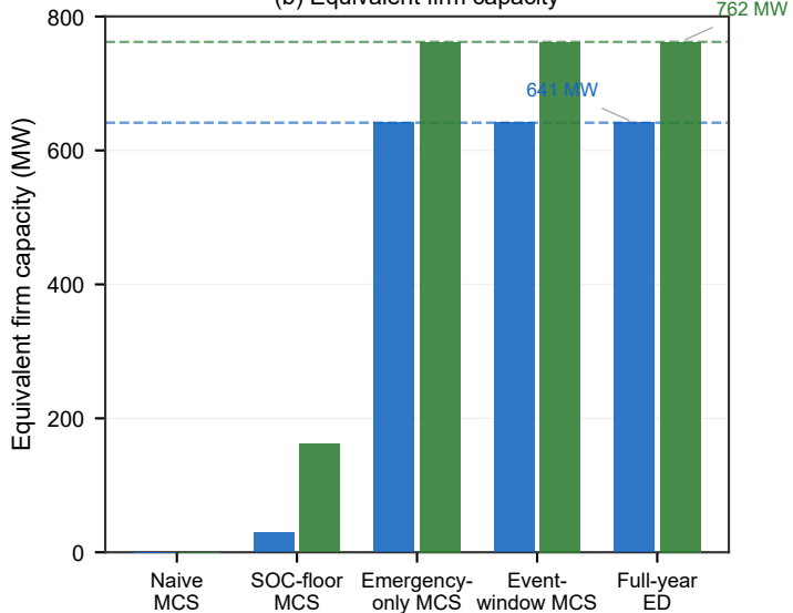
(b) Equivalent firm capacity
