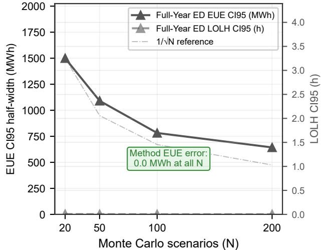
(b) CI95 shrinkage with N
