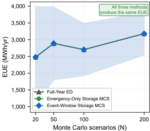
(a) EUE estimates with 95% CI
