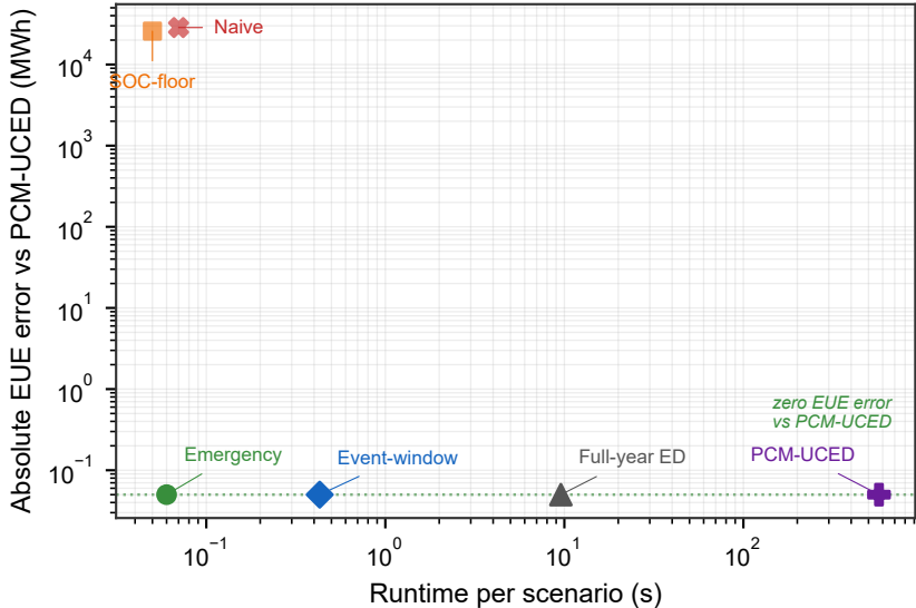
Accuracy–runtime comparison
