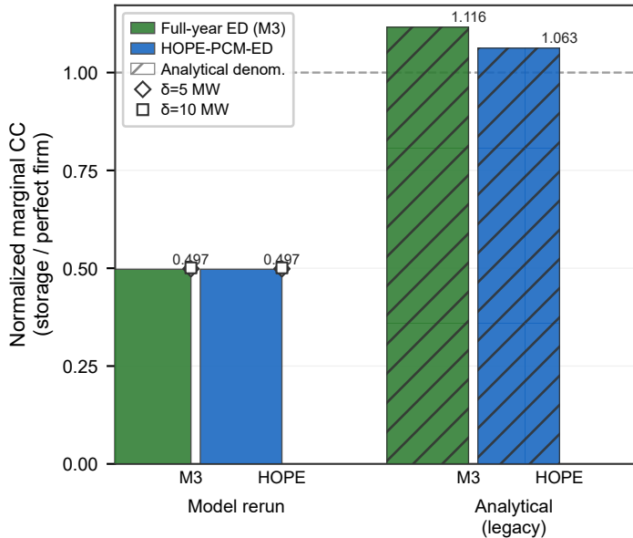
(a) Balanced VRE (N=20)
