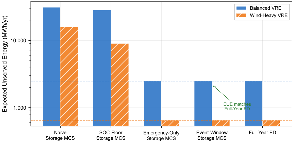
EUE by storage dispatch method
