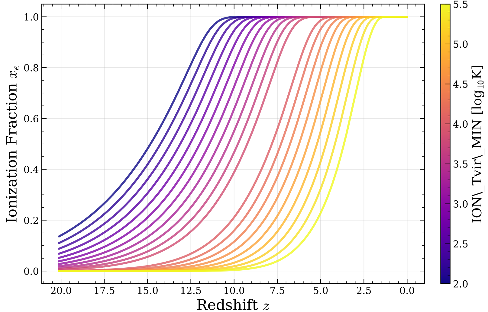
Reionization Histories
