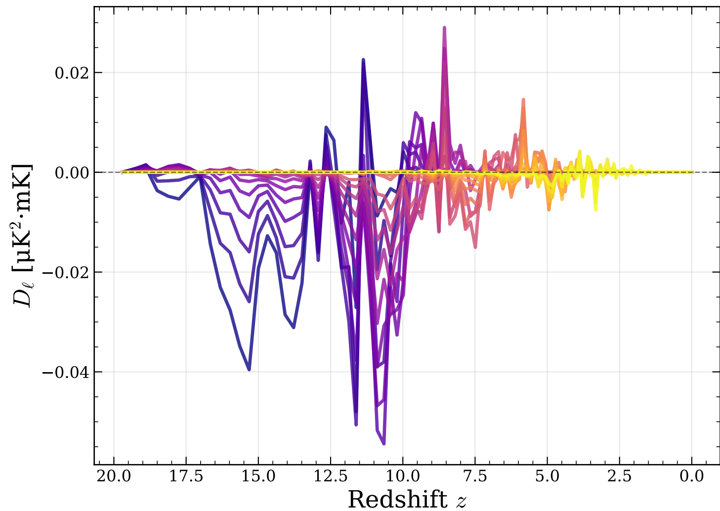
kSZ 2 -21cm Cross-Power at \ell = 1000
