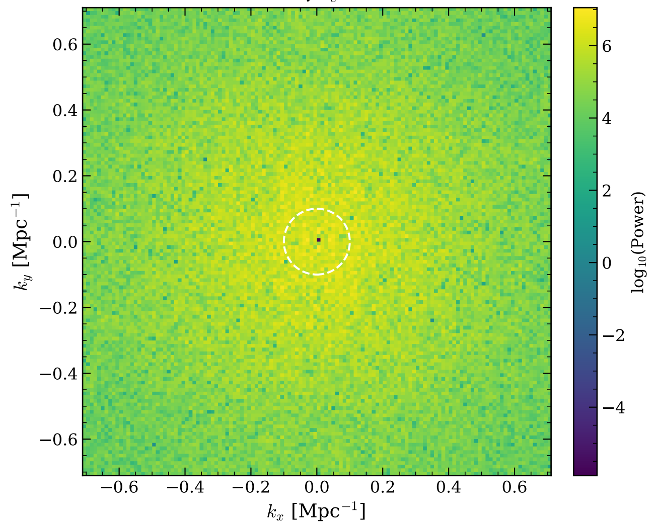
21cm Power (k-space) z=8.01, x_e=0.51
