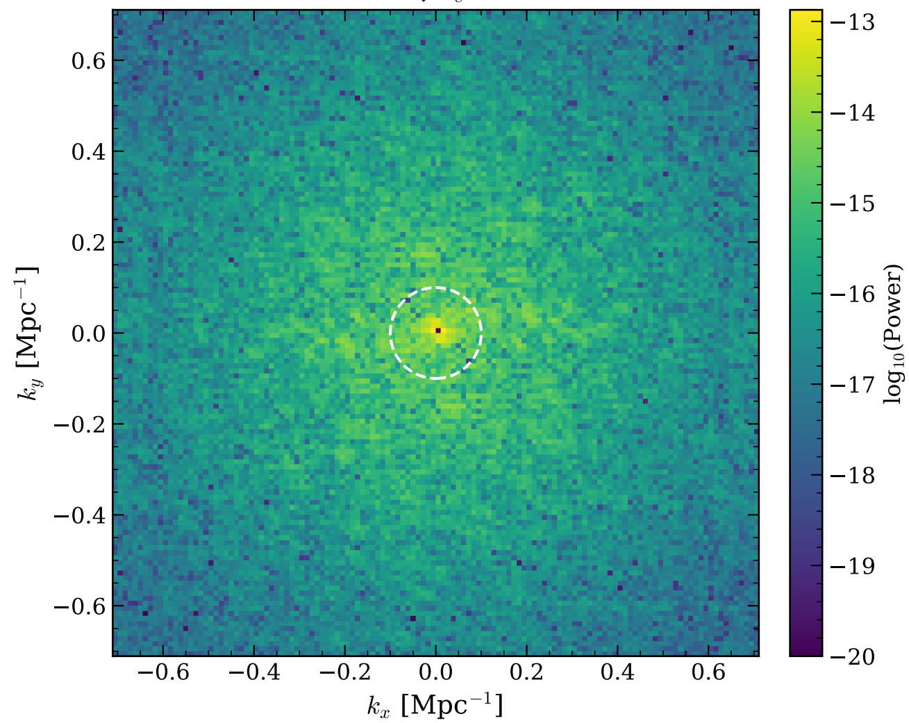
kSZ 2 Power (k-space) z=6.39, x_e=0.90
