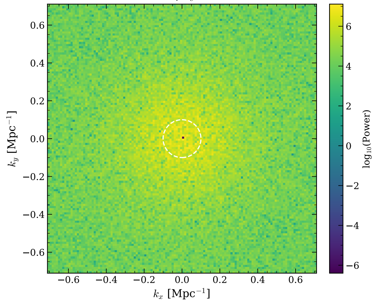
21cm Power (k-space) z=6.39, x_e=0.90
