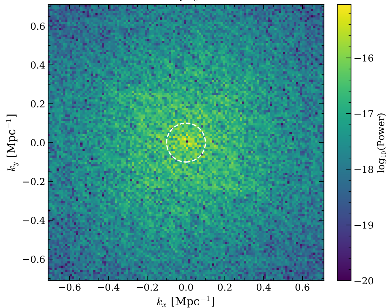
kSZ 2 Power (k-space) z=8.01, x_e=0.51
