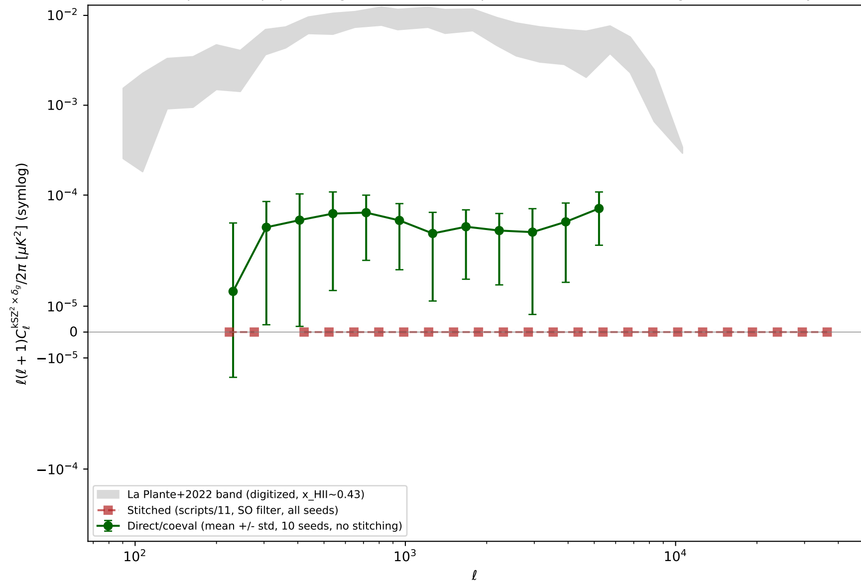
Direct/coeval (lae) vs stitched vs La Plante+2022 -- 10 seeds, z_0=9.5 , dz=1.0 (300 Mpc box vs paper's larger box -- trend/amplitude both shown, nothing normalized away)
