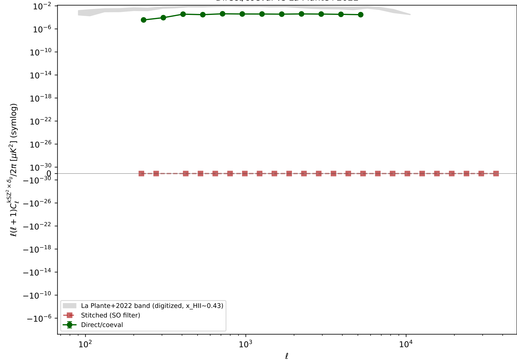
Direct/coeval vs La Plante+2022
