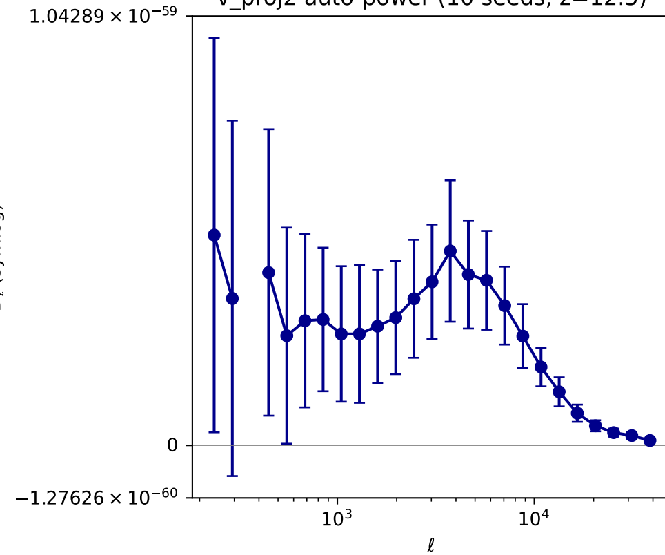
v_proj2 auto-power (10 seeds, z=12.5)
