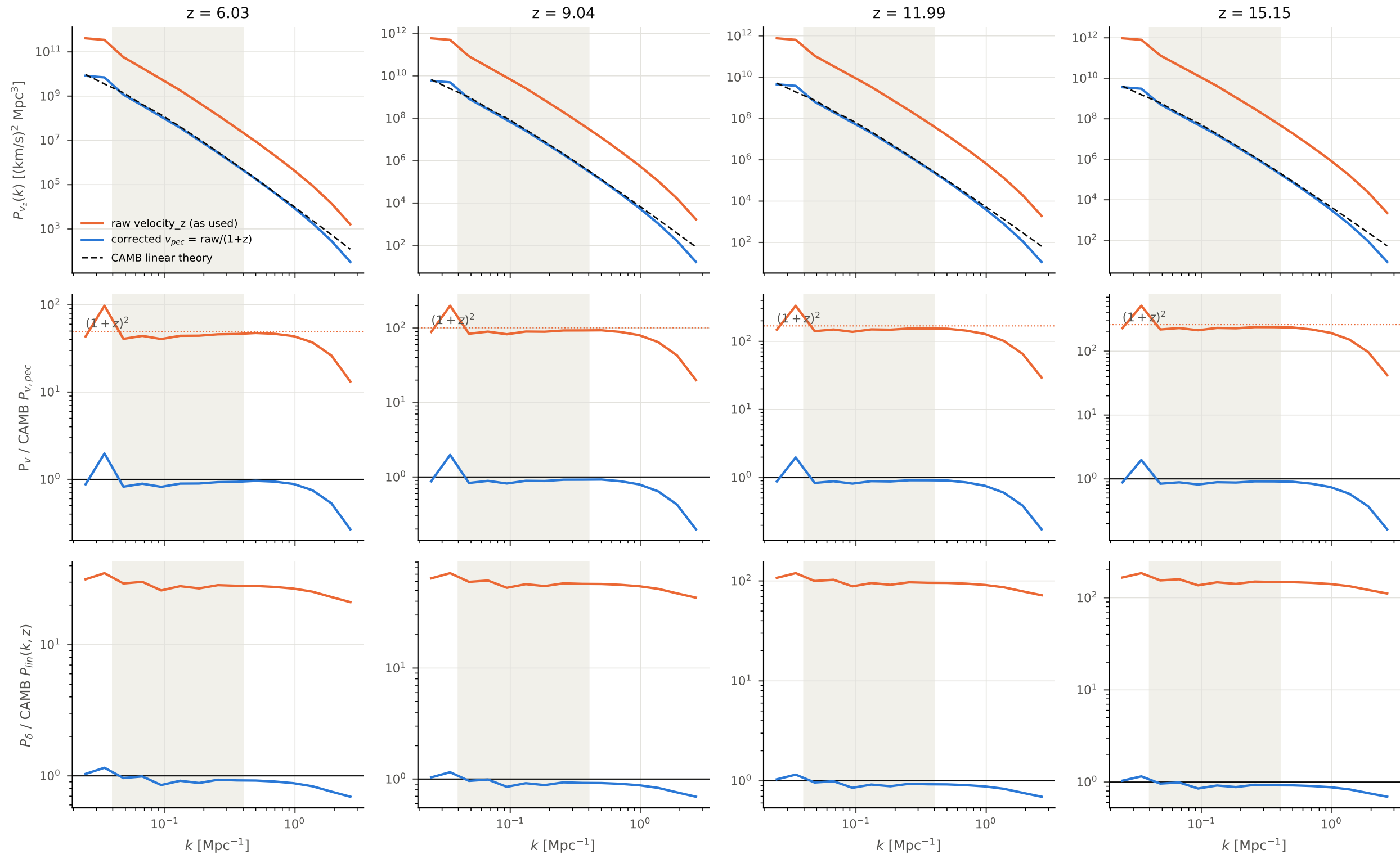
Raw py21cmfast fields vs CAMB linear theory, seed 1 (shaded: linear range k=0.04\text{-}0.4\text{ Mpc}^{-1} ; lowest- k bins have few modes)
