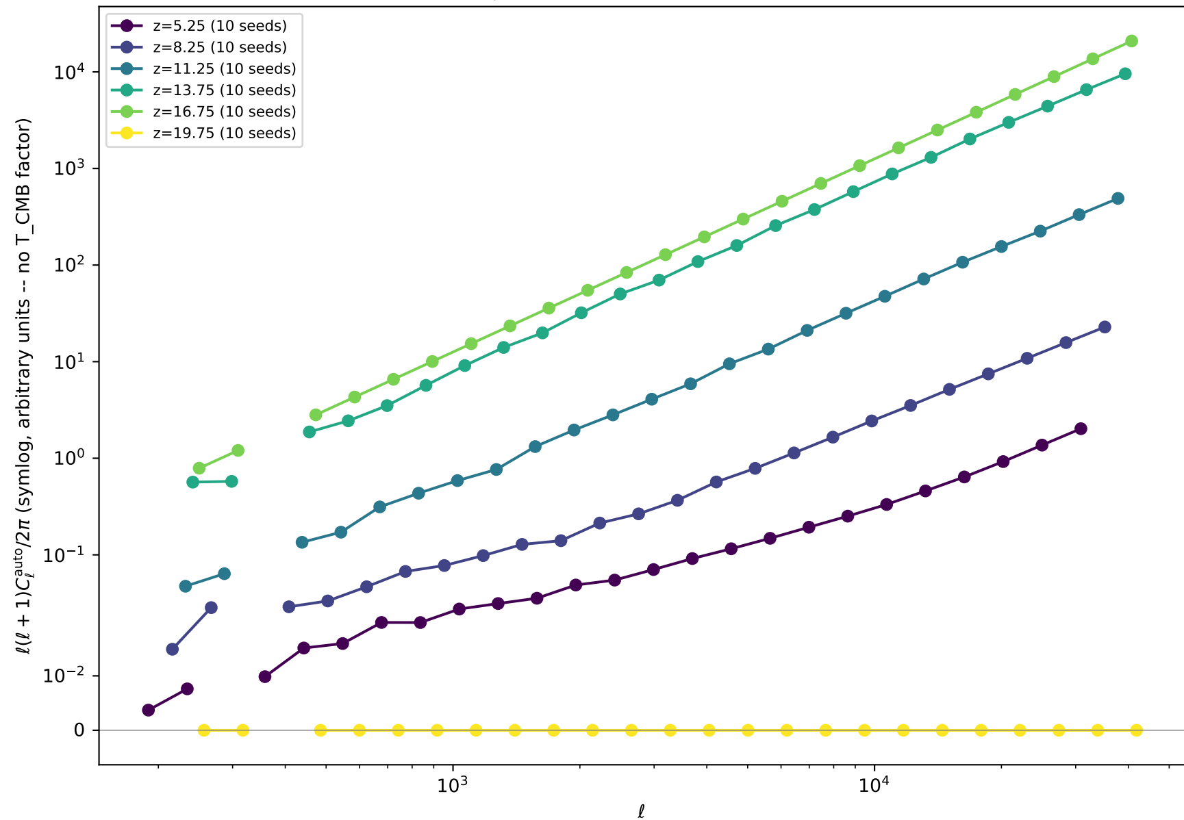
halo auto-power vs ell, at several z (10 seed(s))
