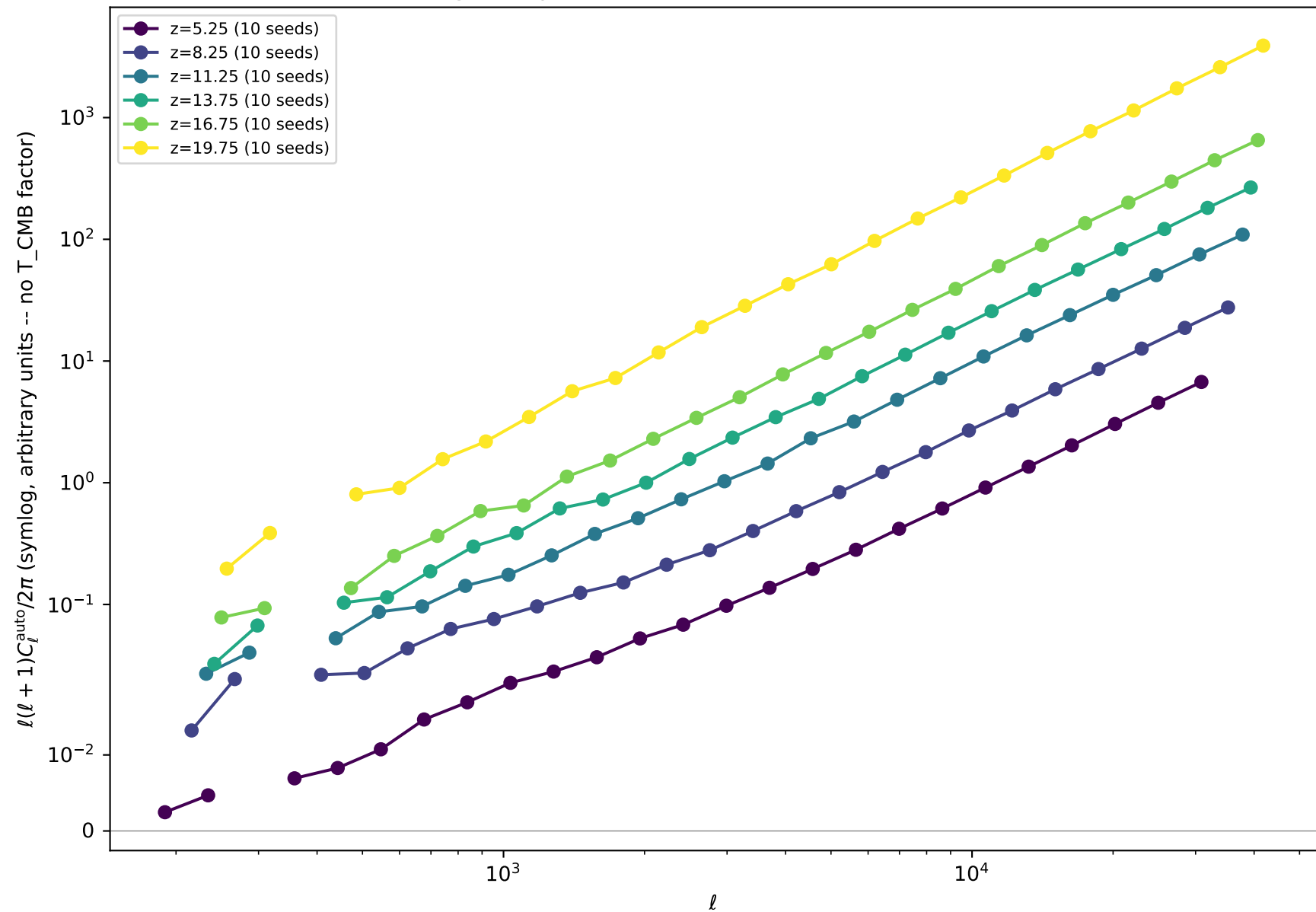
lbg auto-power vs ell, at several z (10 seed(s))
