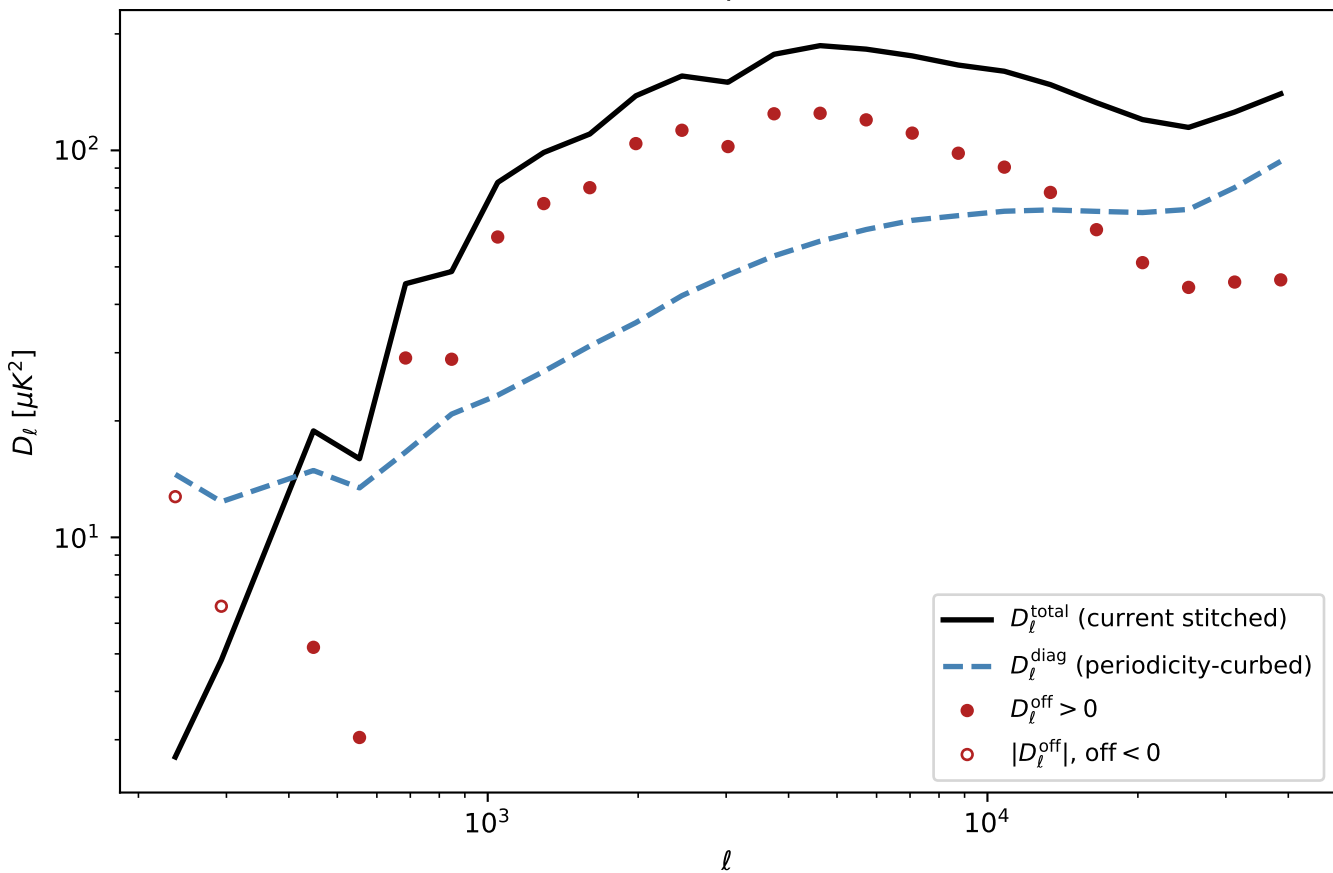
kSZ auto-power coherence decomposition -- seed median_10seeds (300 Mpc box)
