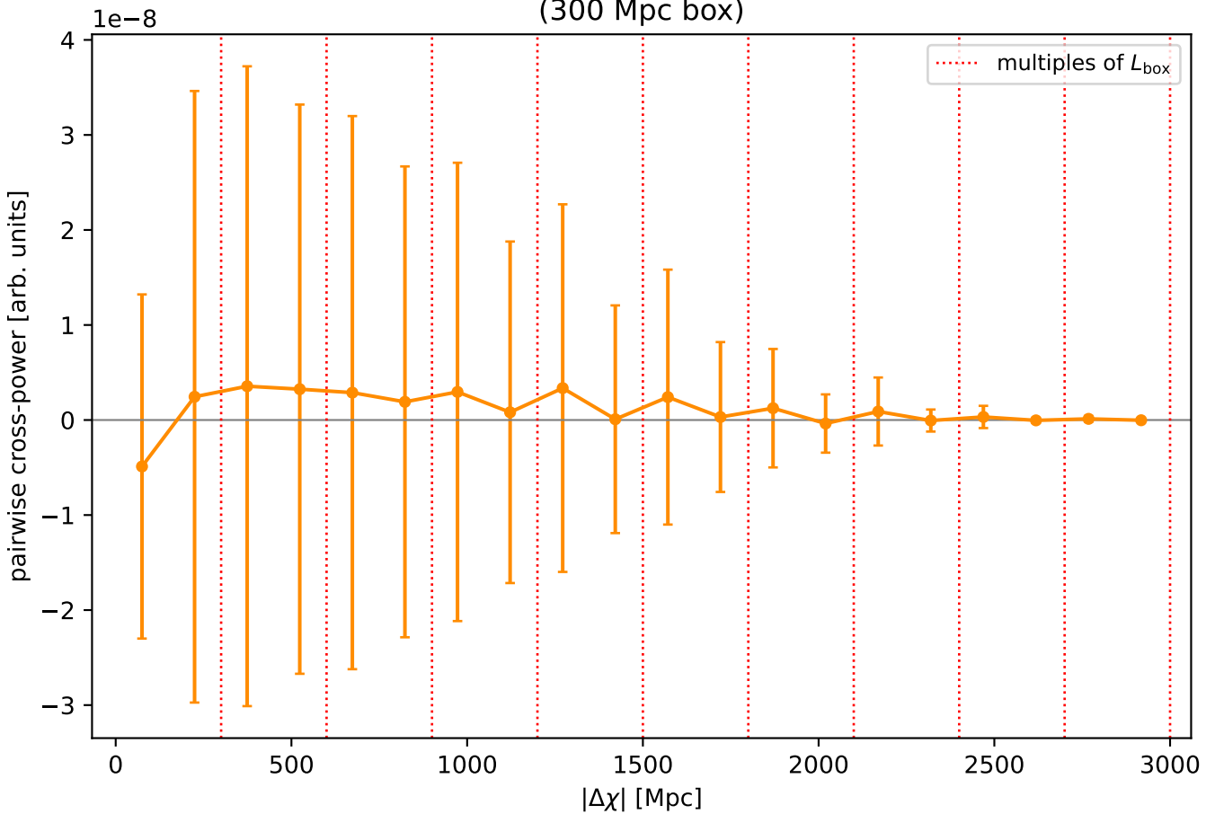
Delta-chi periodicity check -- seed 1 (300 Mpc box)
