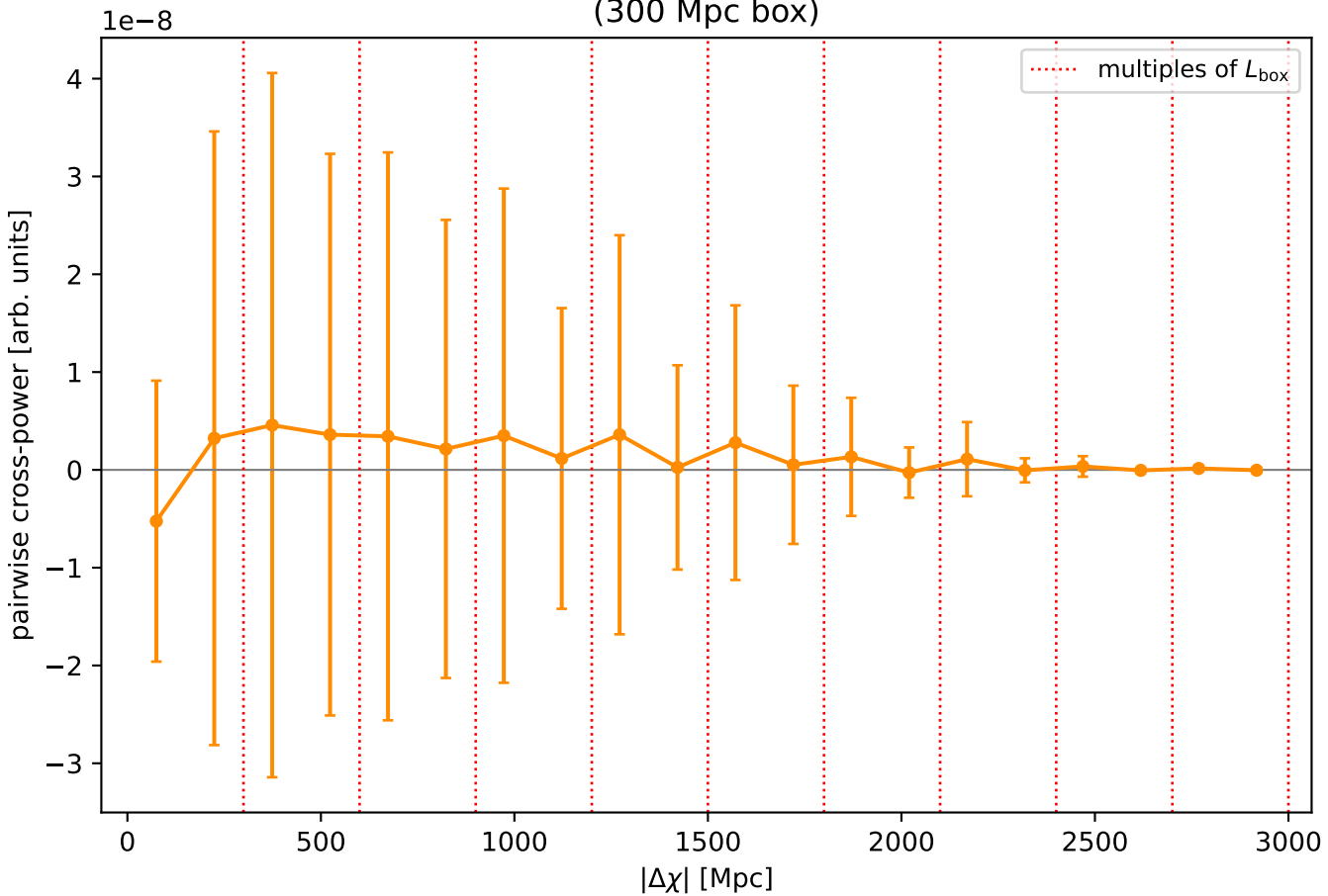
Delta-chi periodicity check -- seed 9 (300 Mpc box)
