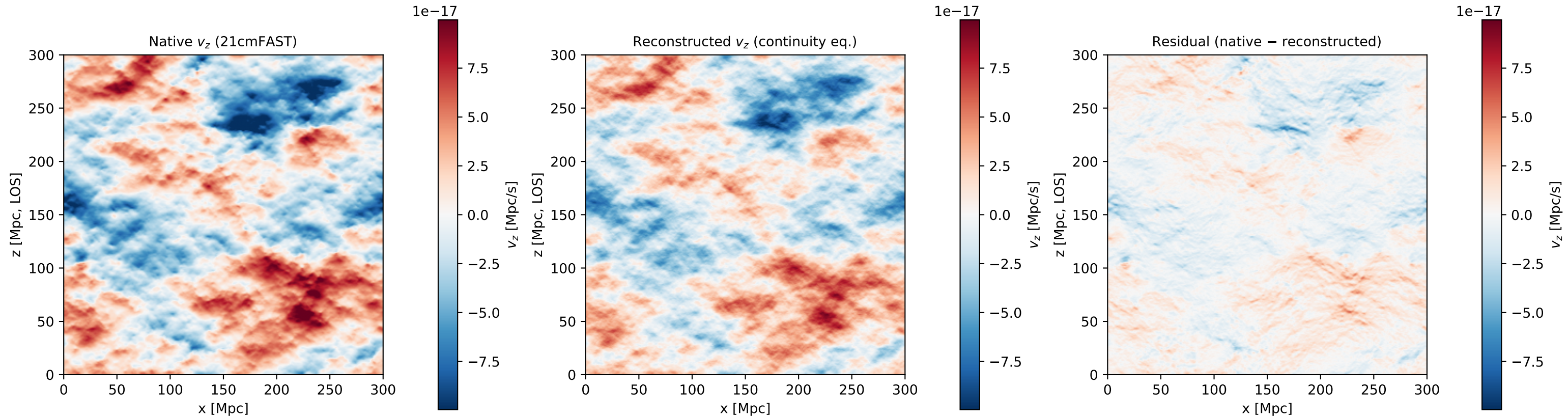
Velocity slice comparison -- seed 1, z=10.307 (y-index=150 of 300, matter field, bias=1.0)
