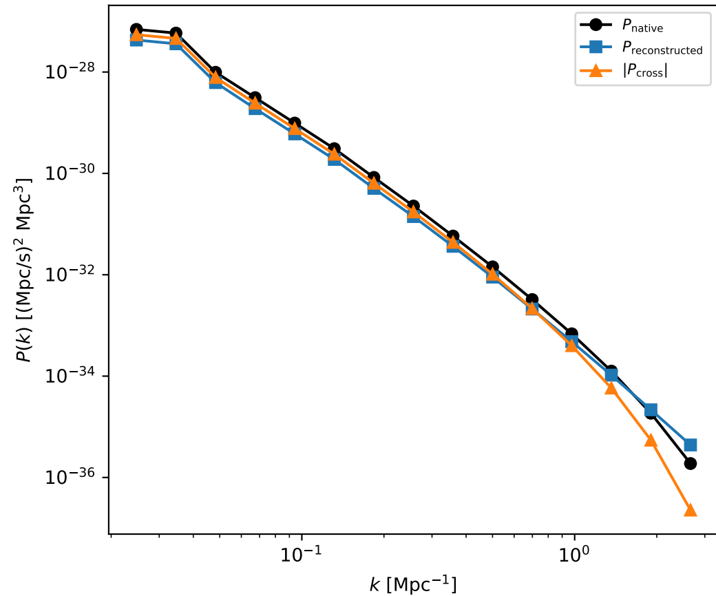
Power spectra (seed 1, z=10.31)
