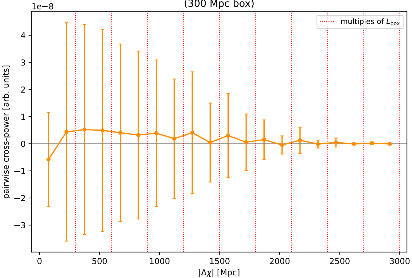
Delta-chi periodicity check -- seed 3 (300 Mpc box)
