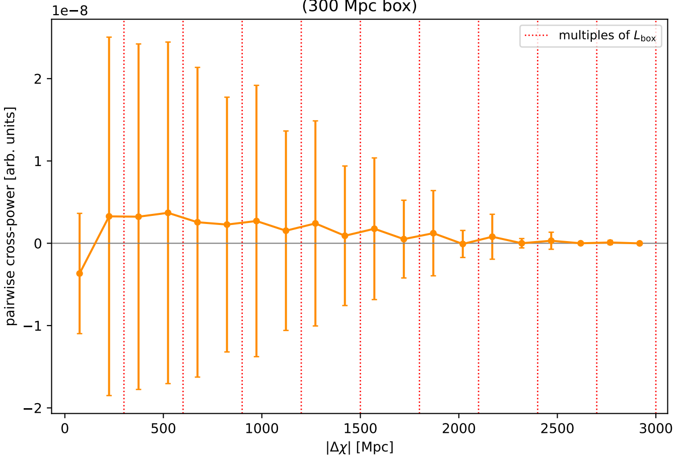
Delta-chi periodicity check -- seed 4 (300 Mpc box)
