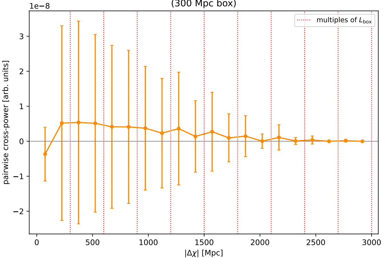
Delta-chi periodicity check -- seed 6 (300 Mpc box)
