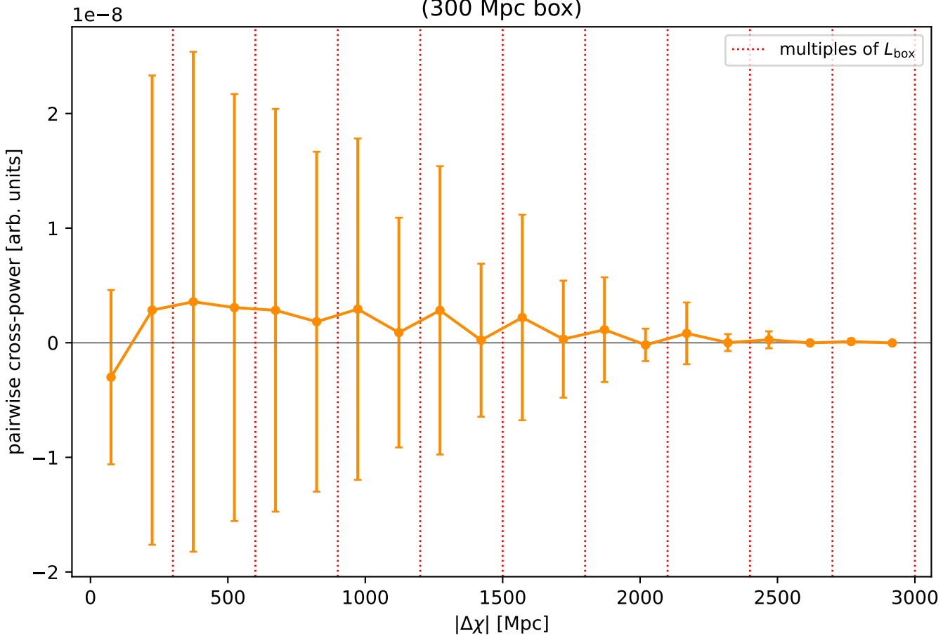
Delta-chi periodicity check -- seed 8 (300 Mpc box)
