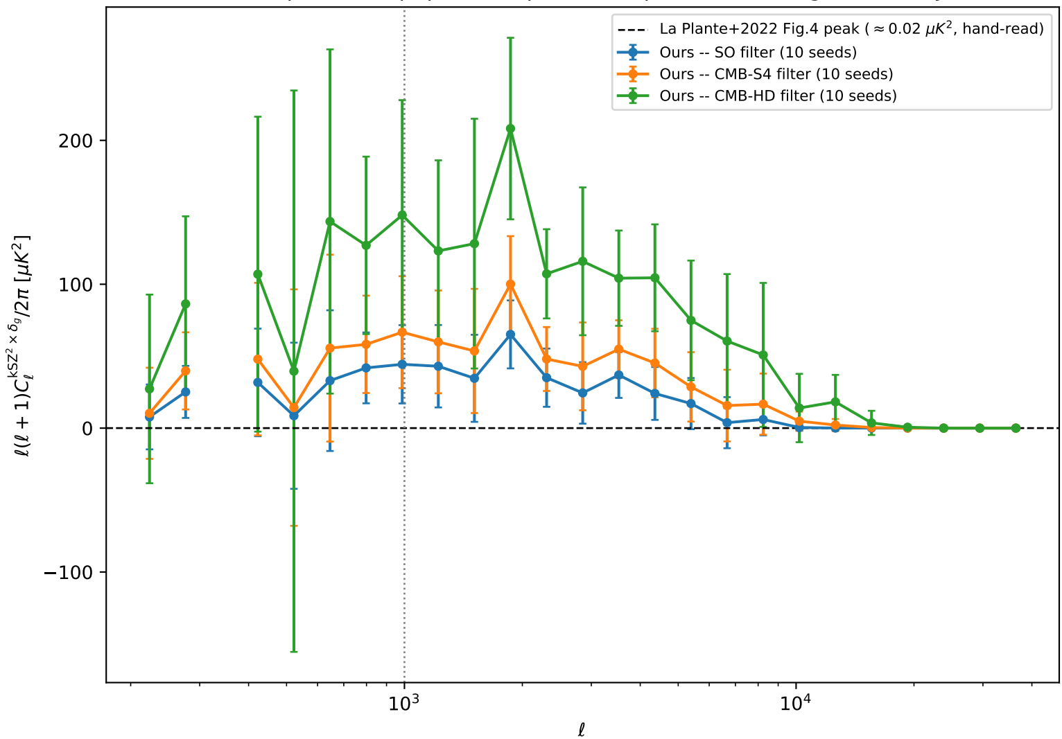
Stage 1 comparison -- z_0=9.5 , dz=1.0 (300 Mpc box vs paper's 2 Gpc/h -- shape/order-of-magnitude only)
