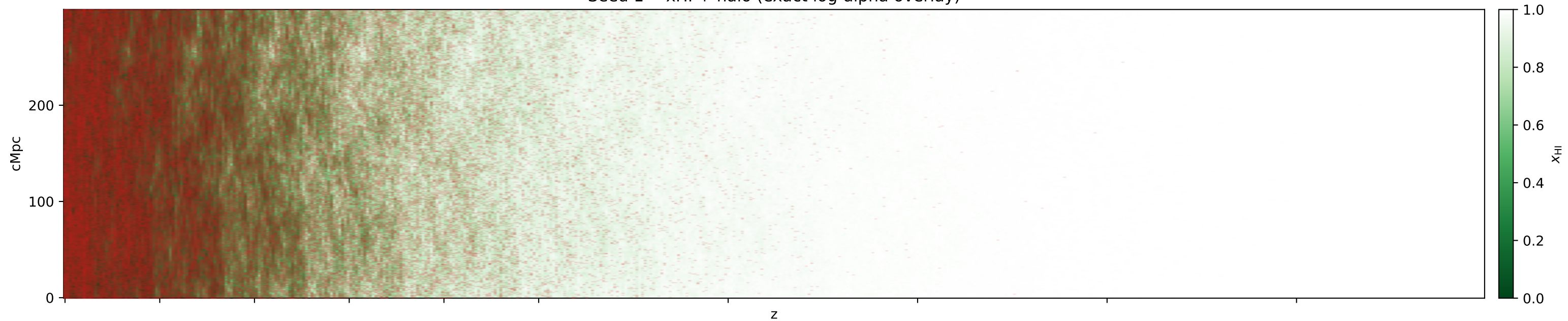
Seed 1 -- xHI + lae (exact log-alpha overlay)
