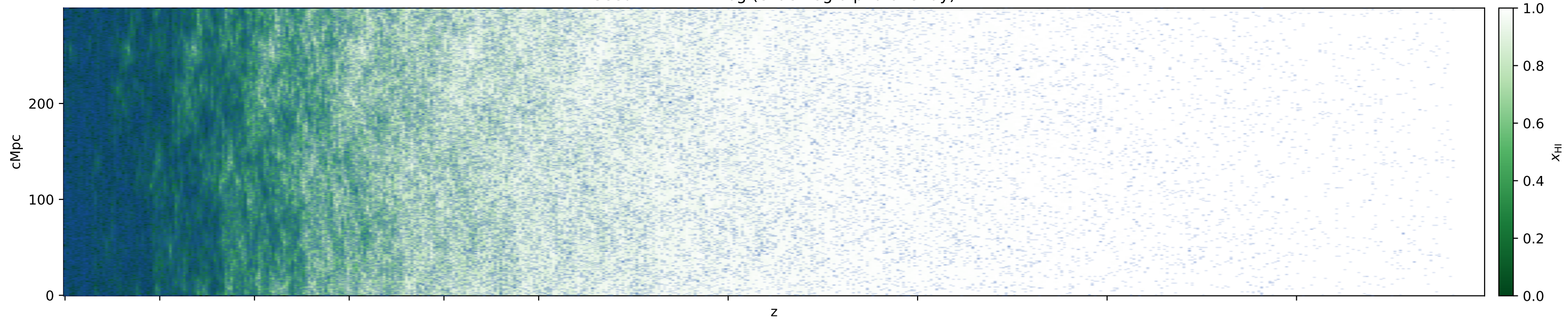
Seed 1 -- xHI + all tracers (exact log-alpha overlay)
