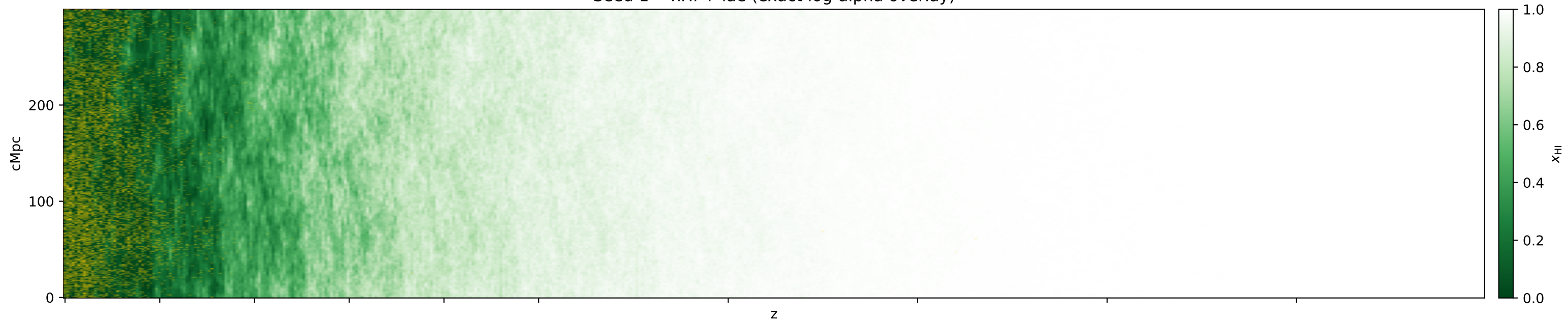
Seed 1 -- xHI + lbg (exact log-alpha overlay)
