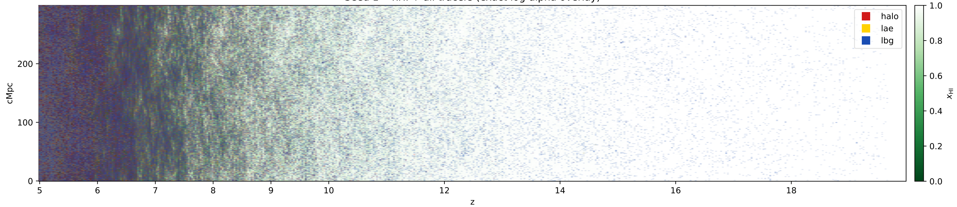
Seed 1 -- xHI + all tracers (exact log-alpha overlay)
