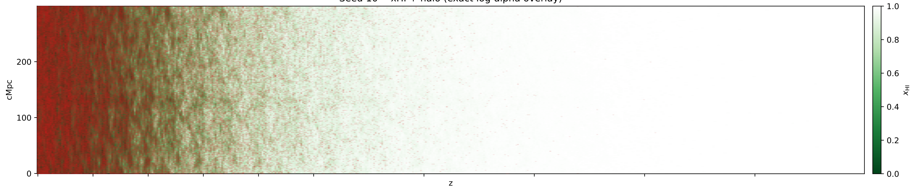
Seed 10 -- xHI + lae (exact log-alpha overlay)
