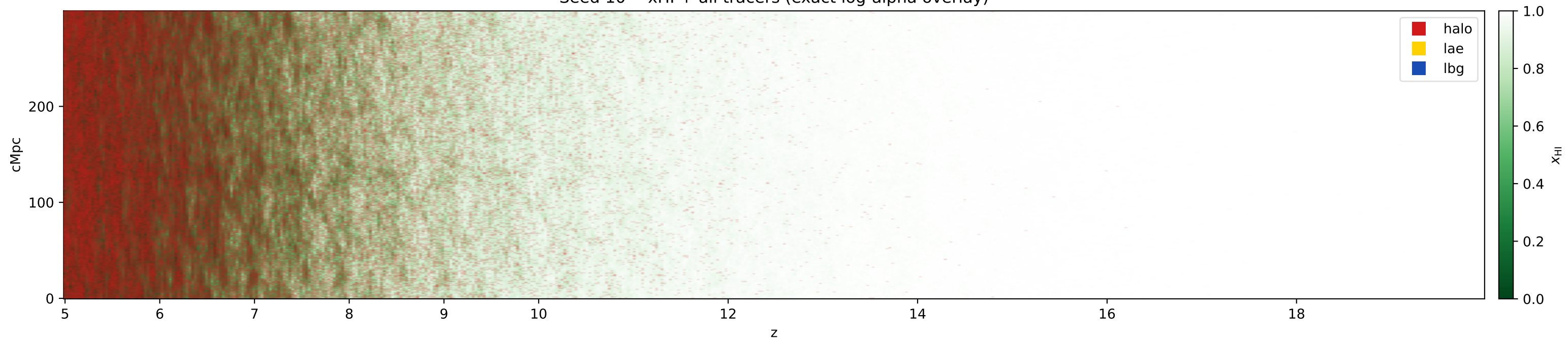
Seed 10 -- xHI + all tracers (exact log-alpha overlay)
