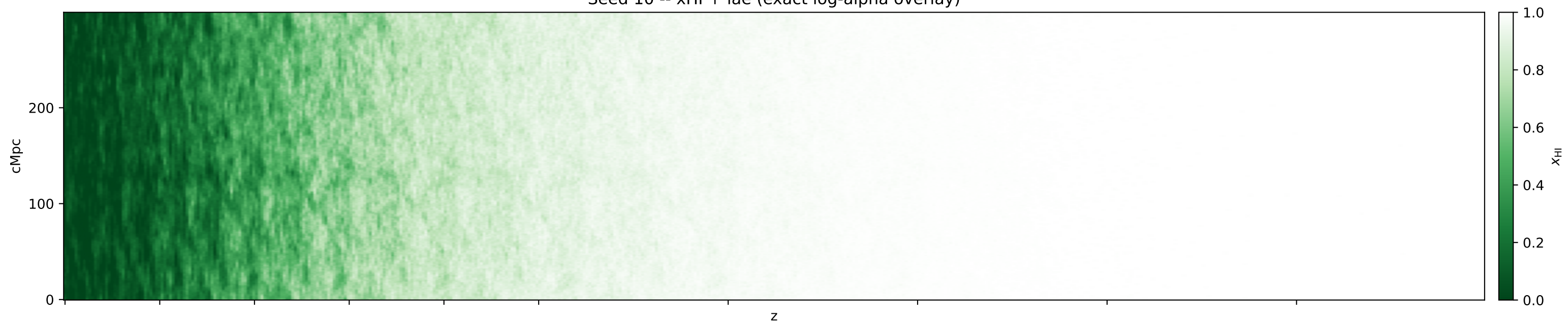
Seed 10 -- xHI + lbg (exact log-alpha overlay)
