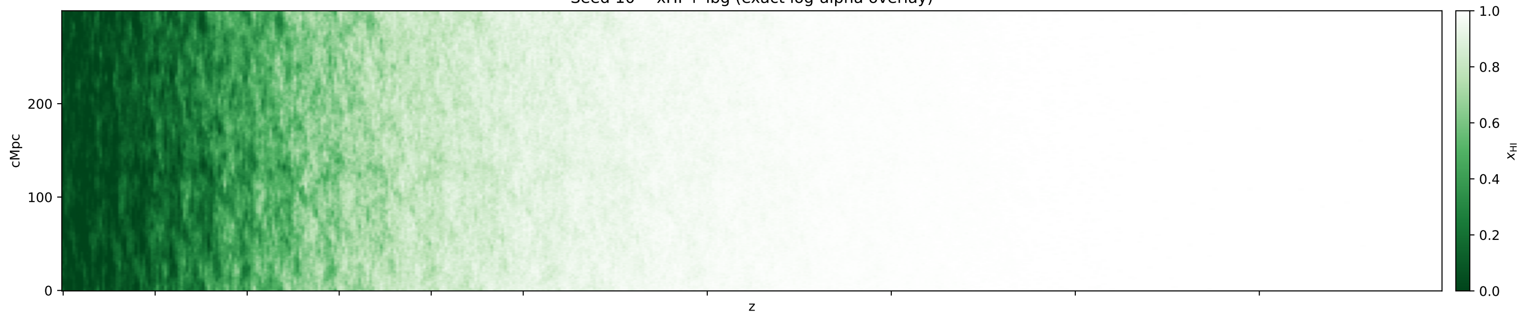
Seed 10 -- xHI + all tracers (exact log-alpha overlay)
