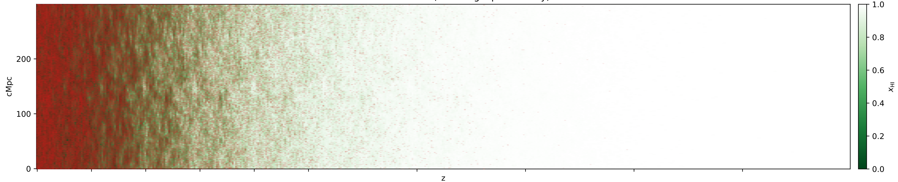
Seed 2 -- xHI + lae (exact log-alpha overlay)
