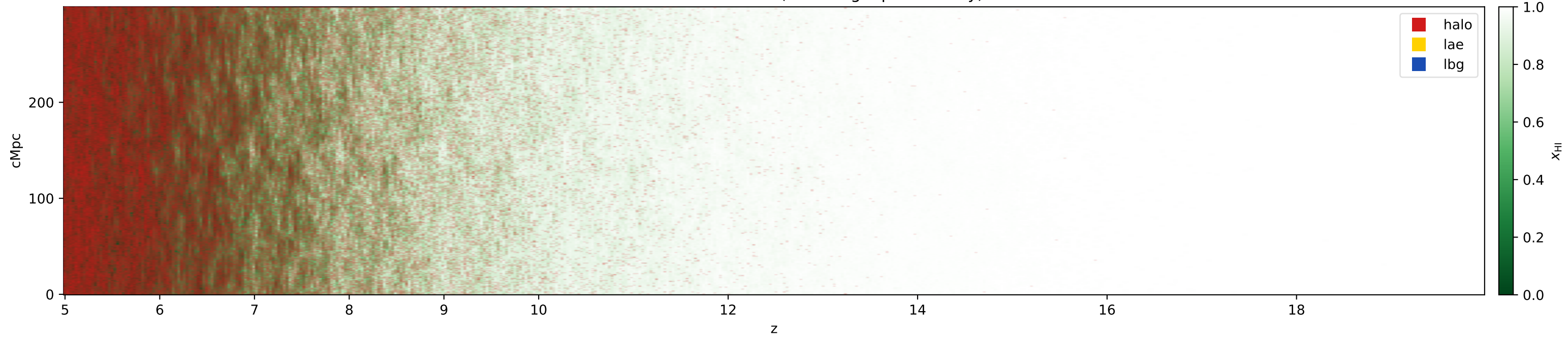
Seed 2 -- xHI + all tracers (exact log-alpha overlay)
