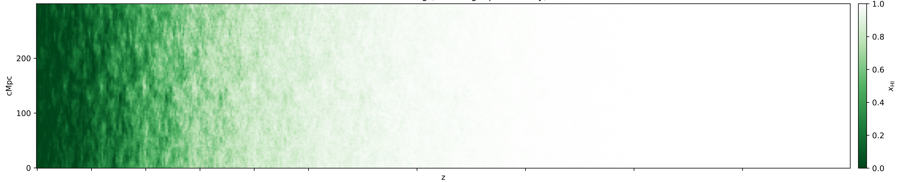
Seed 2 -- xHI + all tracers (exact log-alpha overlay)
