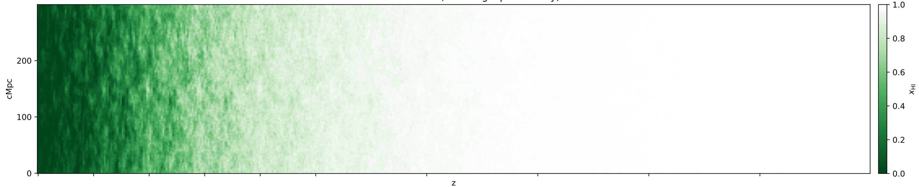
Seed 2 -- xHI + lbg (exact log-alpha overlay)
