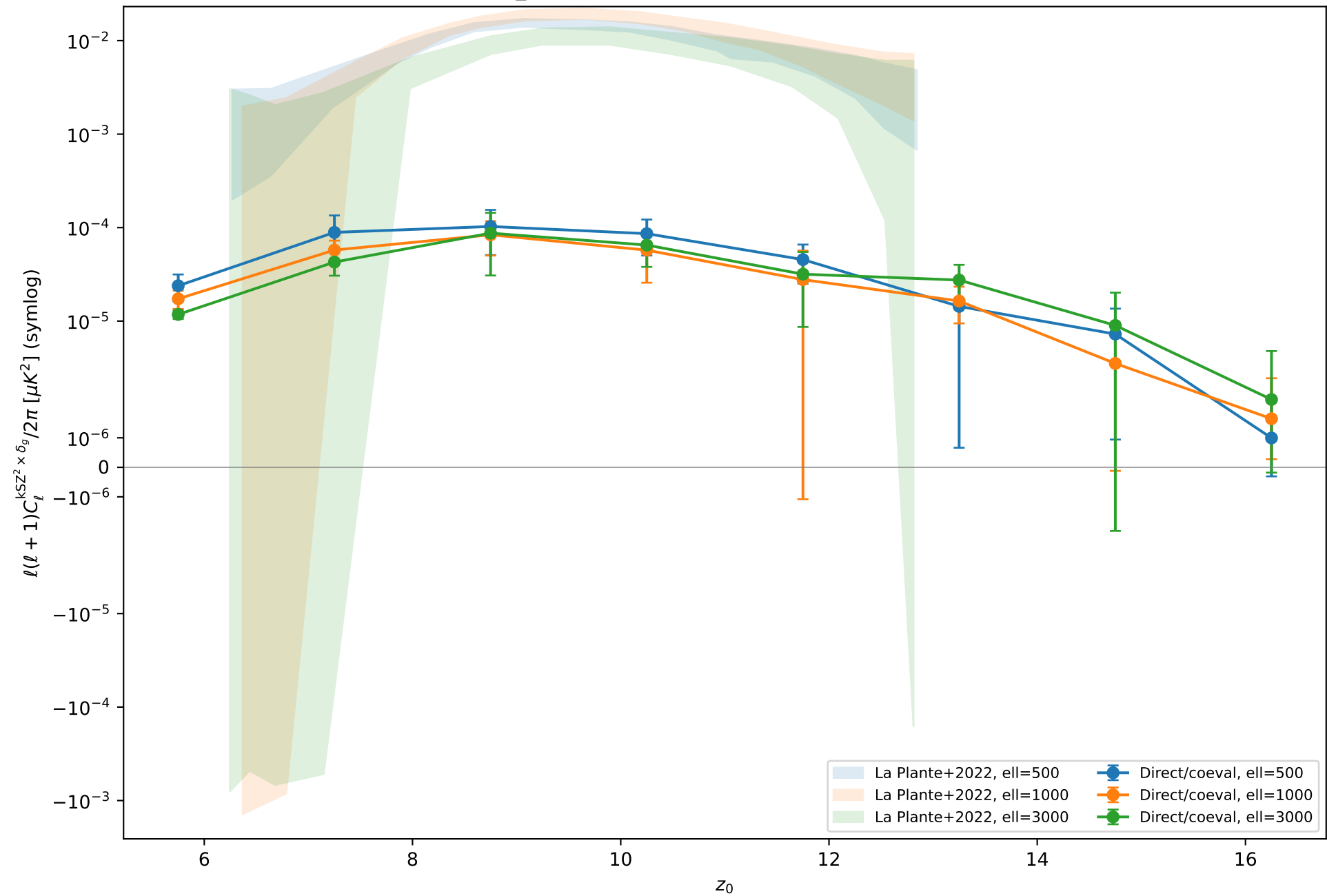
D_ell vs z0, direct/coeval vs La Plante+2022
