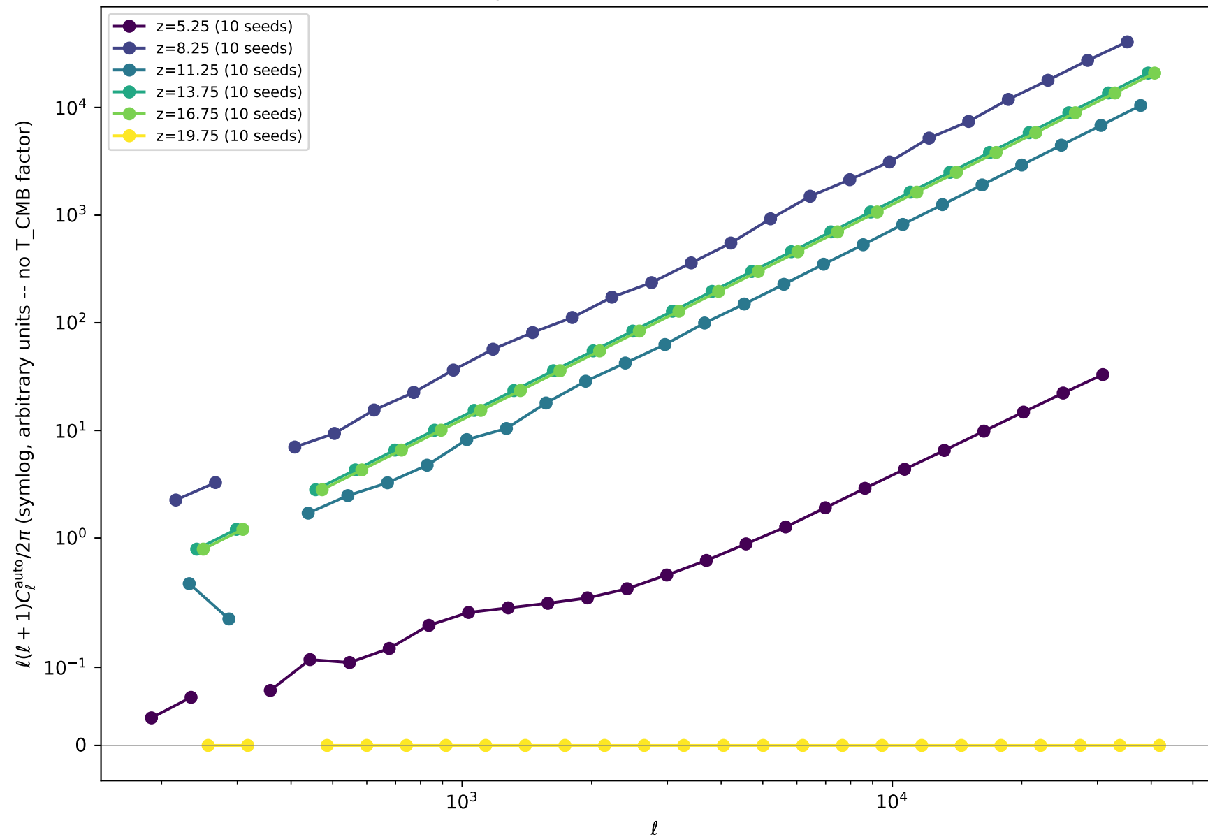
lae auto-power vs ell, at several z (10 seed(s))
