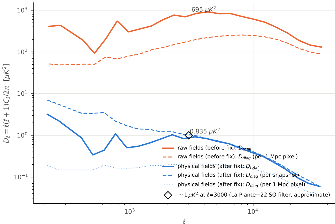
kSZ auto-power, seed 1, patchy window
