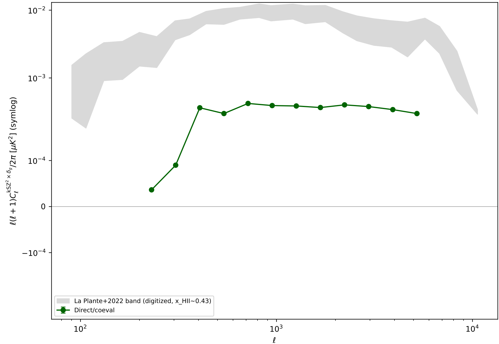
Direct/coeval vs La Plante+2022 (re-plotted from existing CSV)
