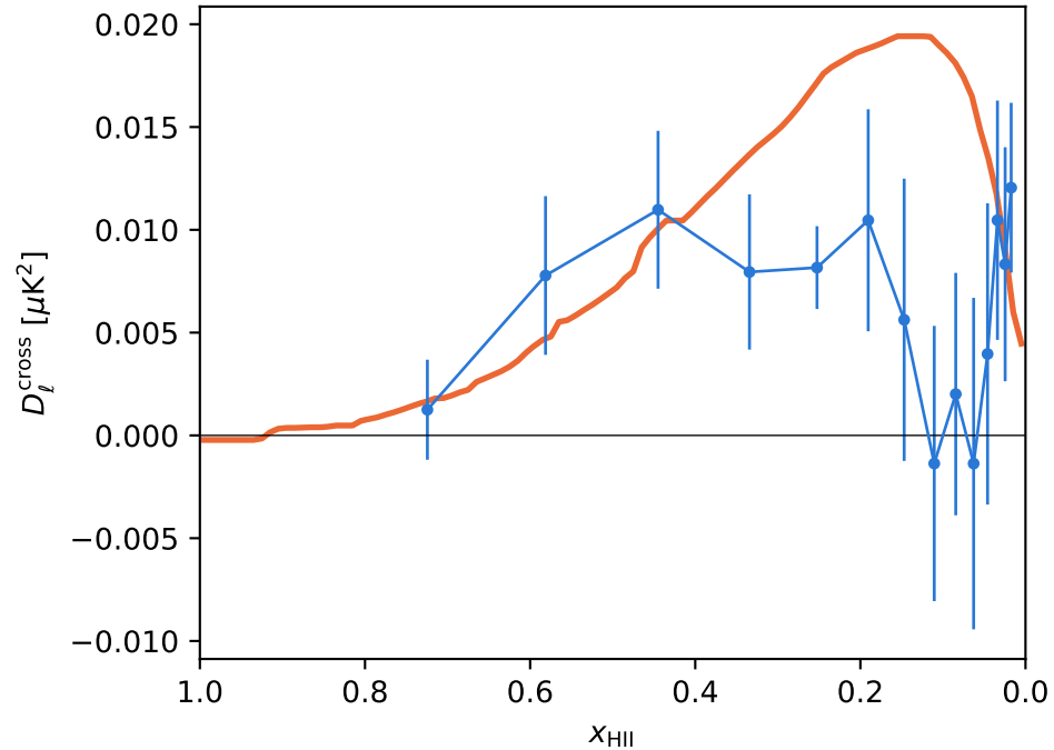
\ell = 1000 (SO)
