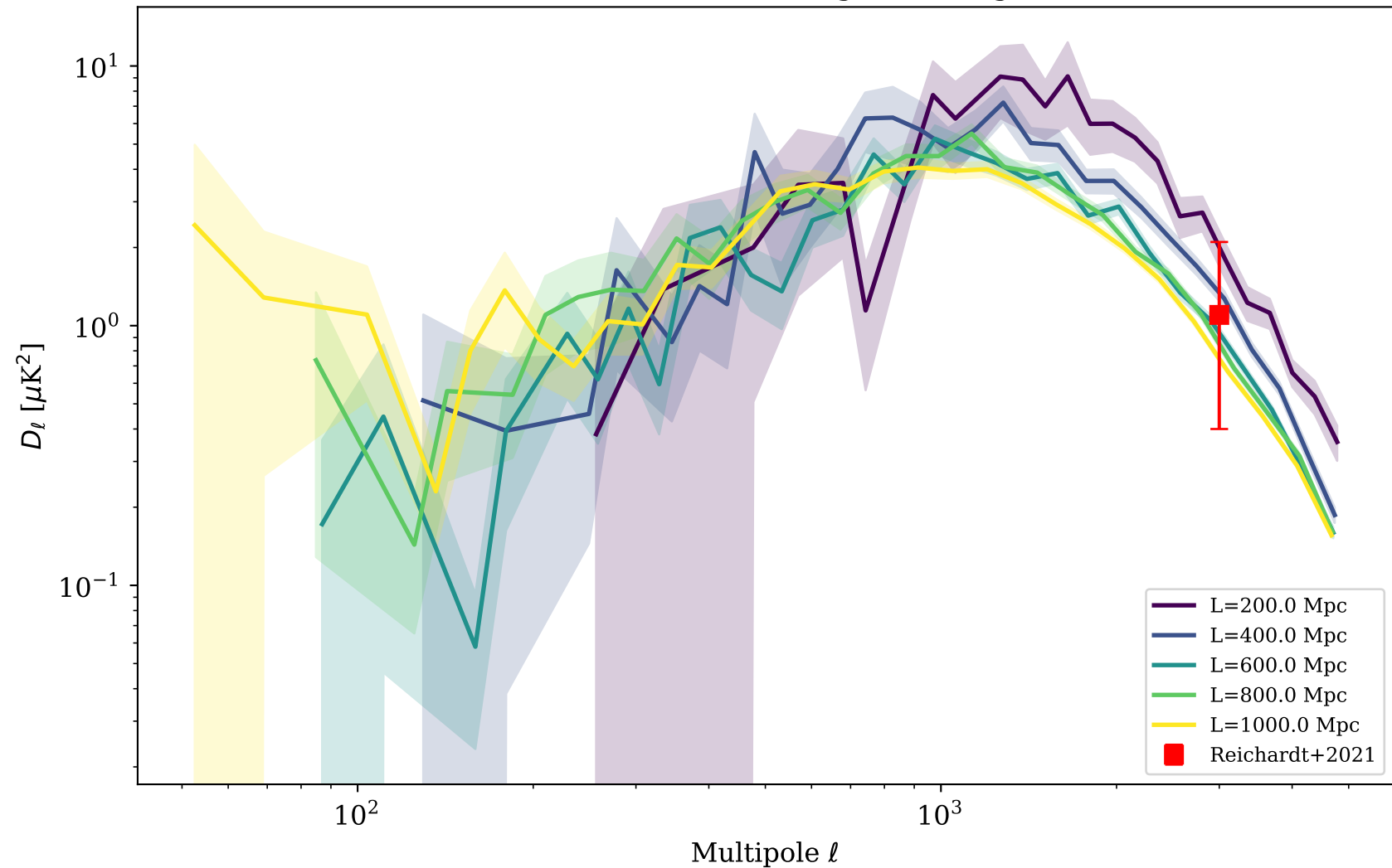
Stitched: box-size convergence, angle=0°
