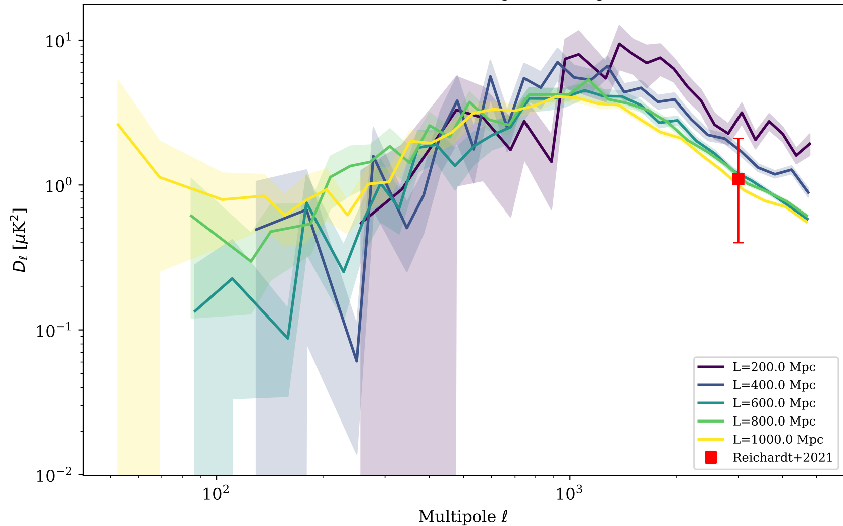
Stitched: box-size convergence, angle=10°
