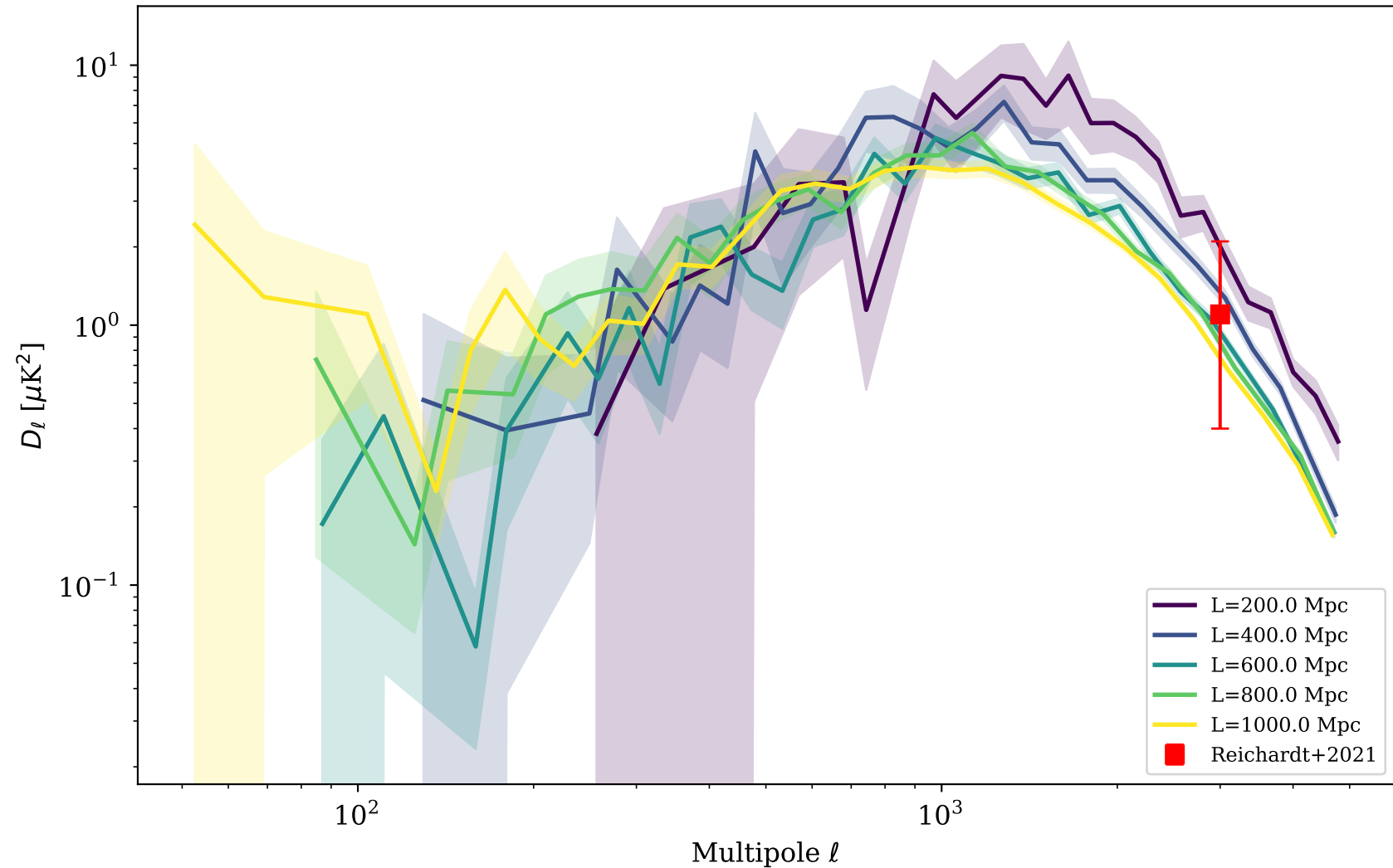
Stitched: box-size convergence (dx=6.25 Mpc fixed)
