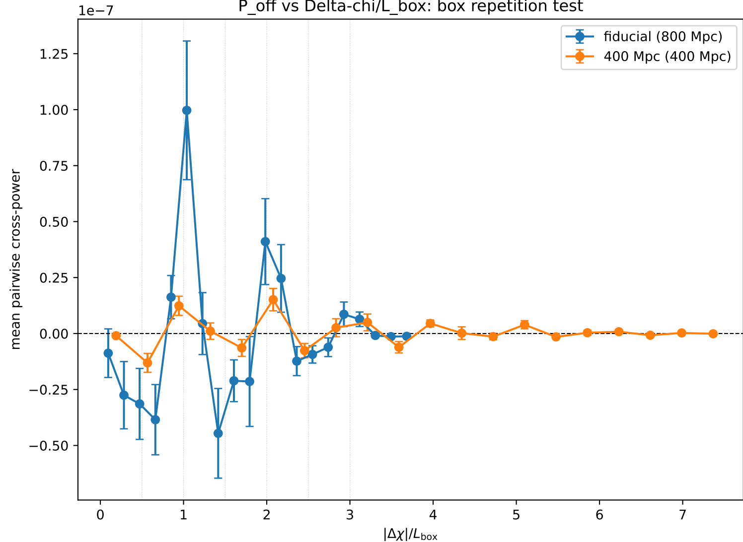
P_{\text{off}} vs \Delta\chi/L_{\text{box}} : box repetition test
