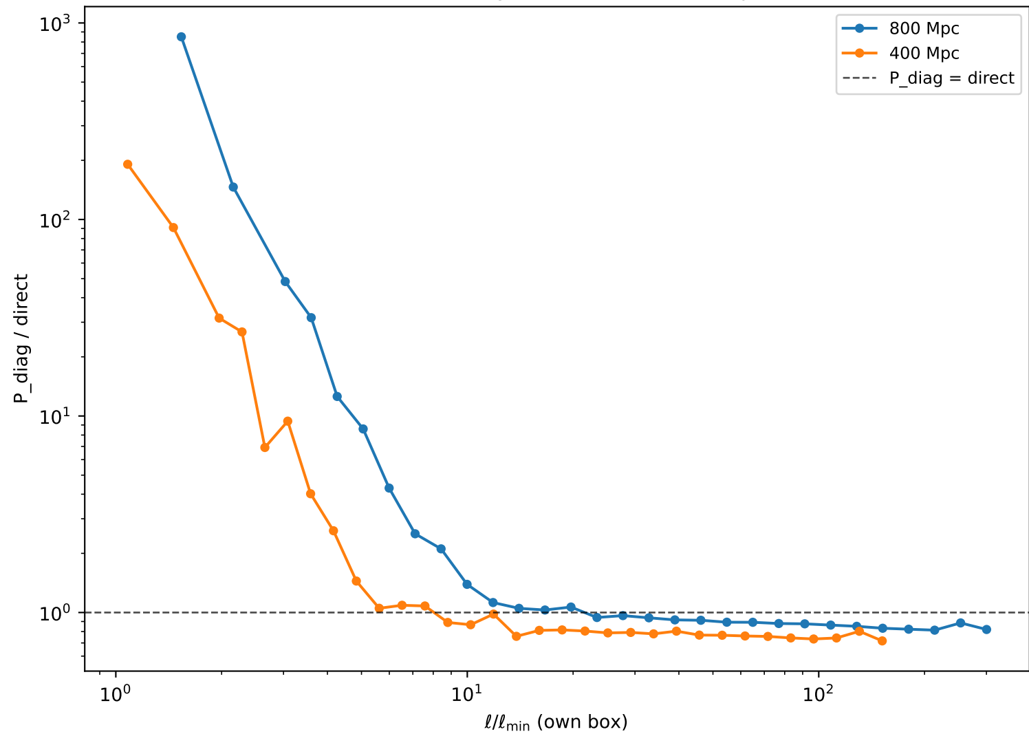
Low-ell excess, normalized by each box's own sample-variance floor
