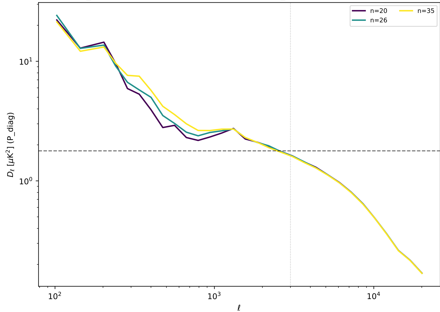
P_diag full spectrum, overlaid across the n_groups=[15,40] plateau
