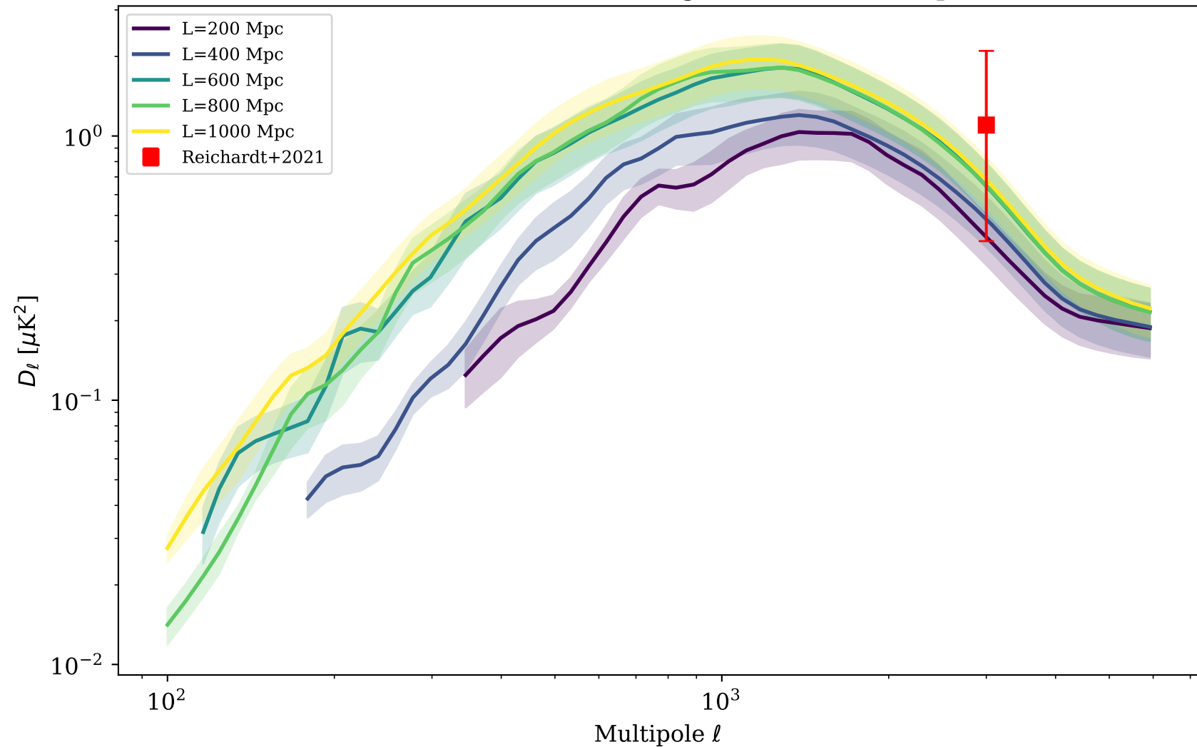
Coeval-direct: box-size convergence (dx=6.25 Mpc fixed)
