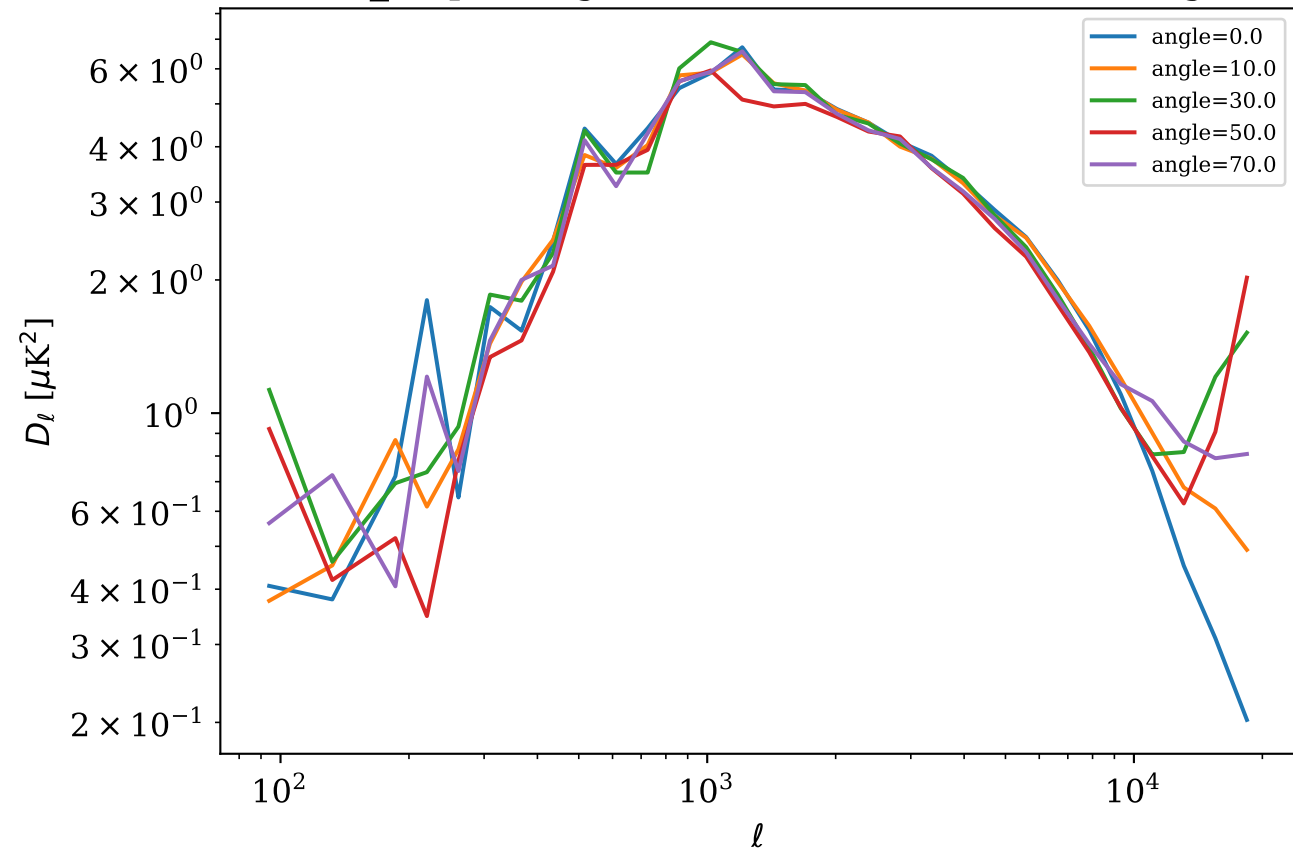
Full D_{\ell} per angle -- watch the \ell \sim 130 -180 region
