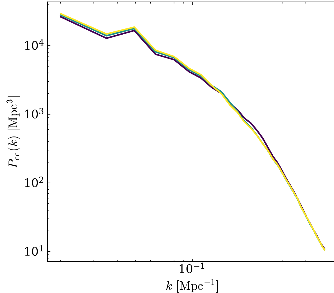
P_{ee} at z=8
