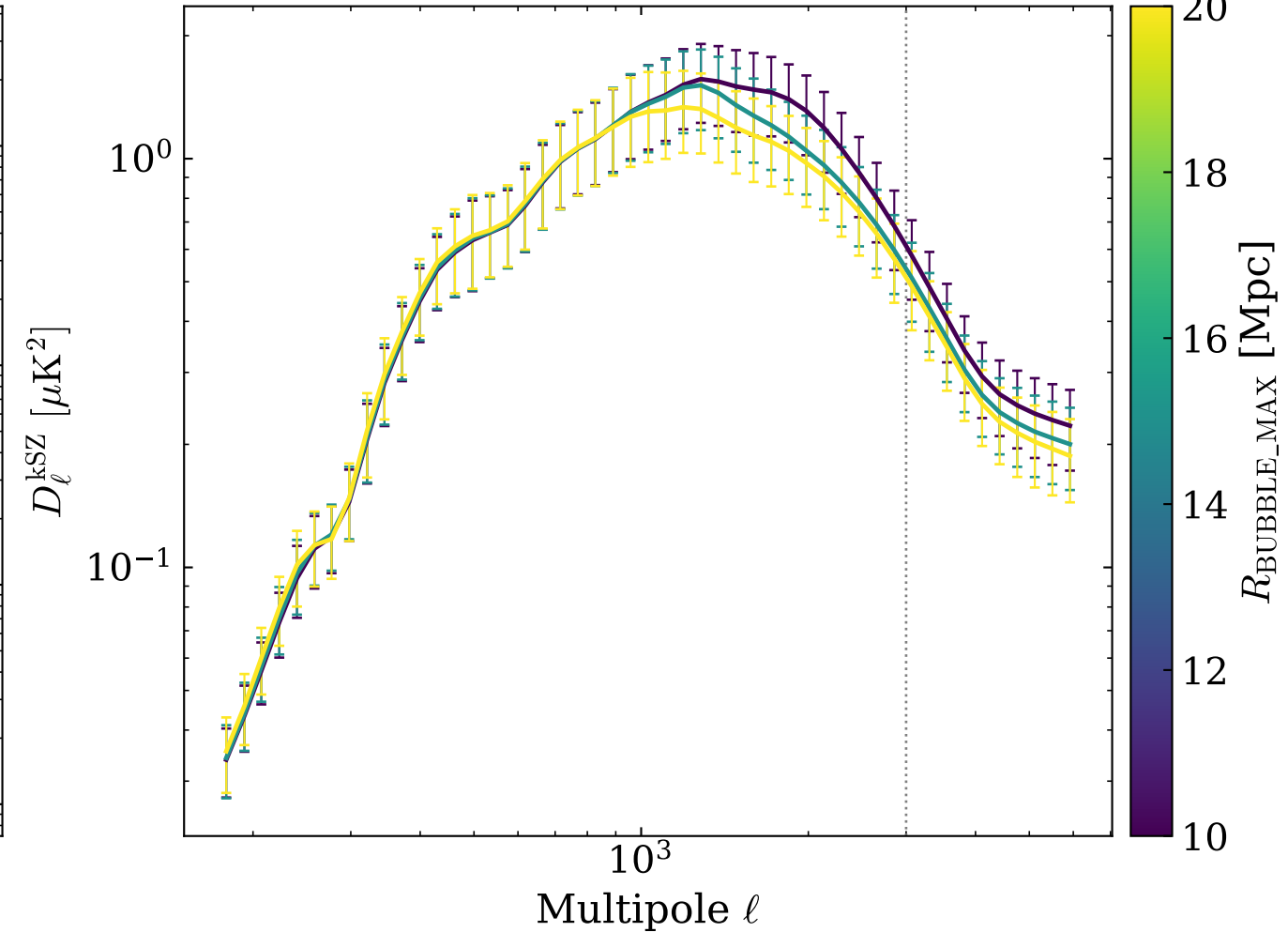
kSZ power (direct/coeval + Limber)
