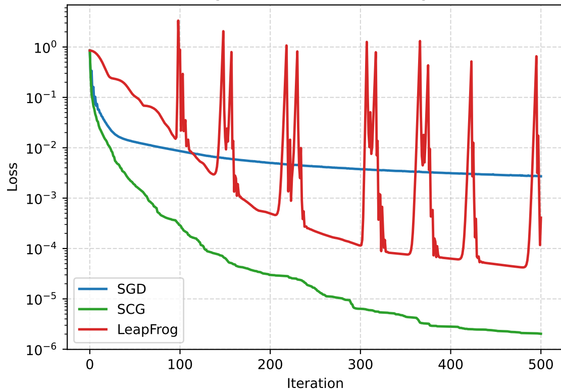
Convergence Curves: Wine Recognition
