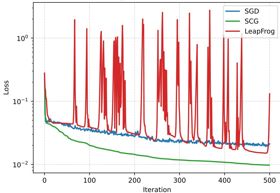
Convergence Curves: Two Moons
