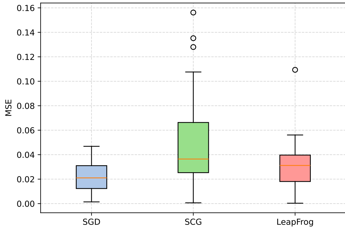
Test MSE (30 Runs)
