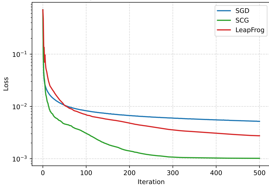
Convergence Curves: Breast Cancer Wisconsin
