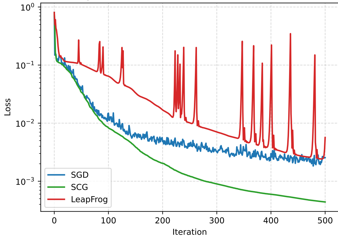
Convergence Curves: Friedman 1 Non-Linear Benchmark
