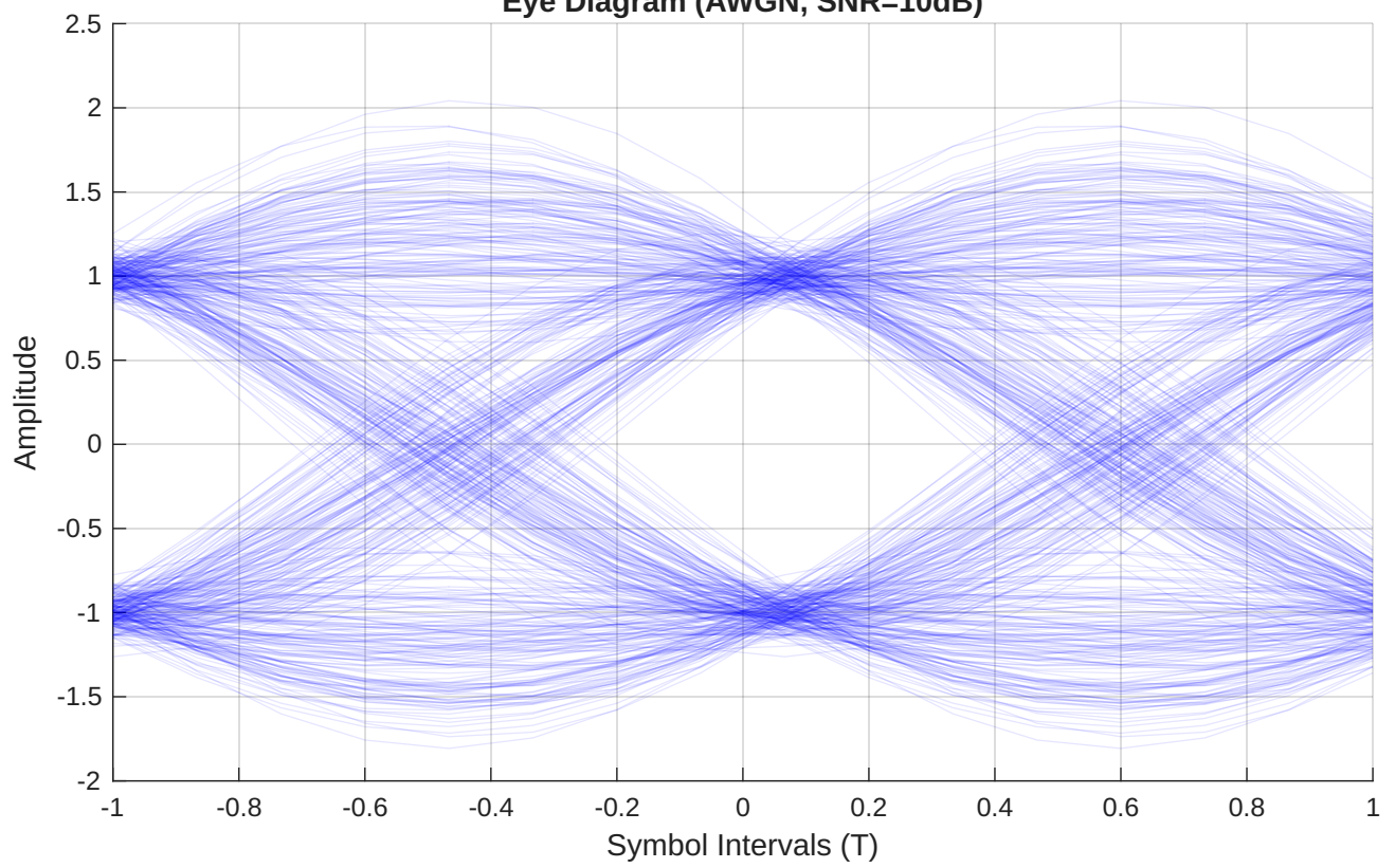
Eye Diagram (AWGN, SNR=10dB)
