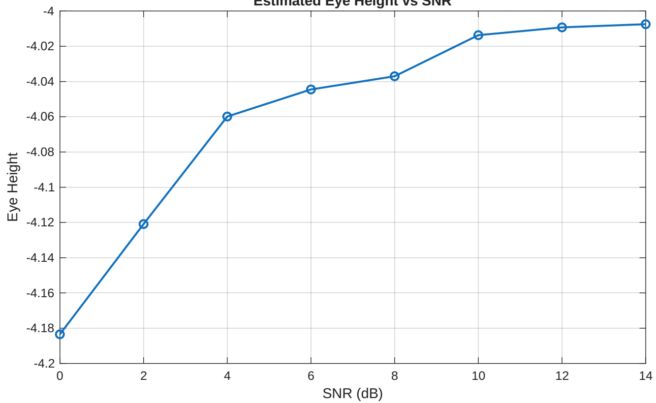
Estimated Eye Height vs SNR
