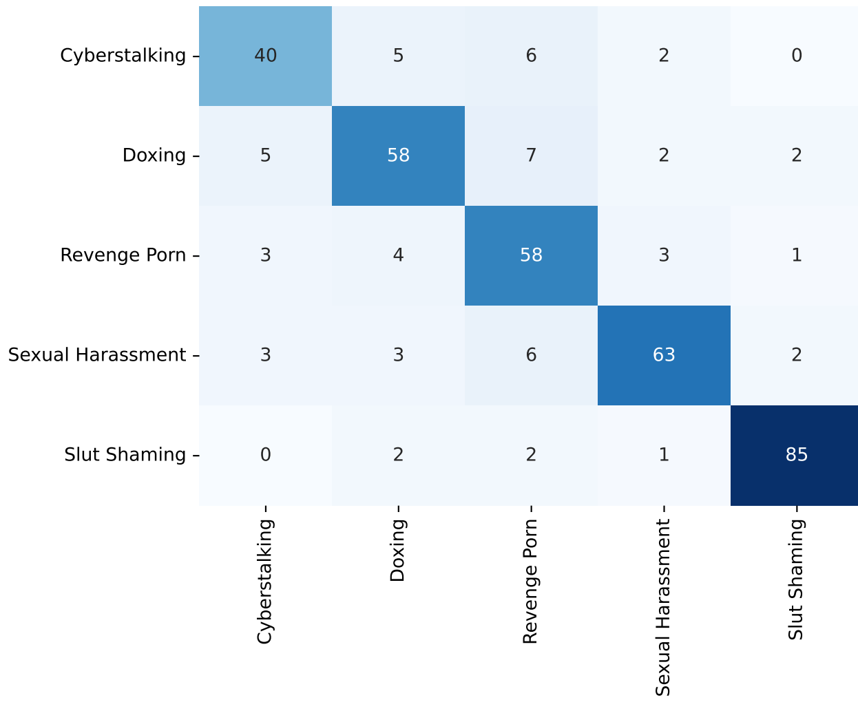
Confusion Matrix
