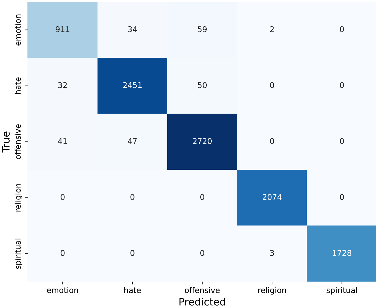
Confusion Matrix
