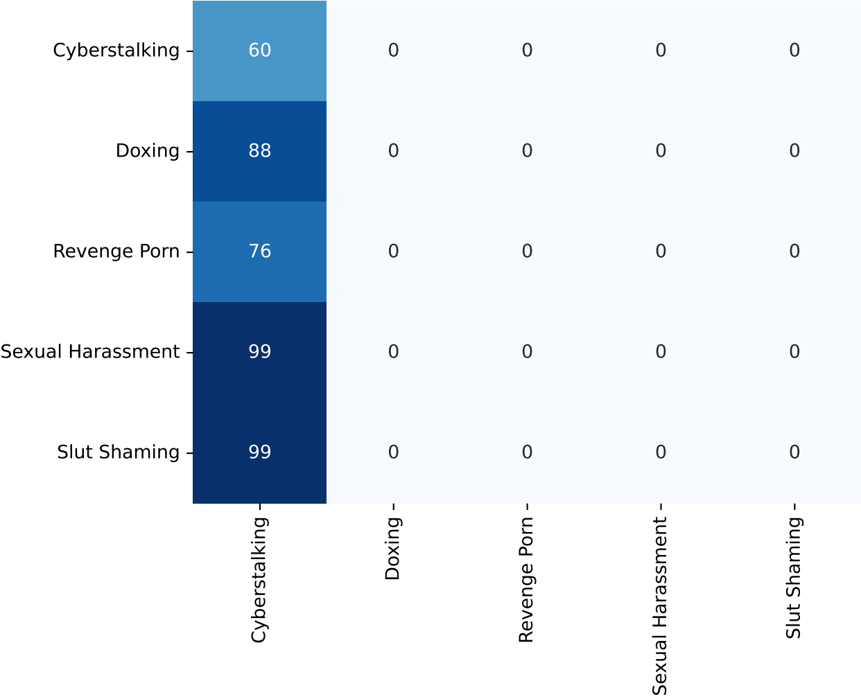
Confusion Matrix
